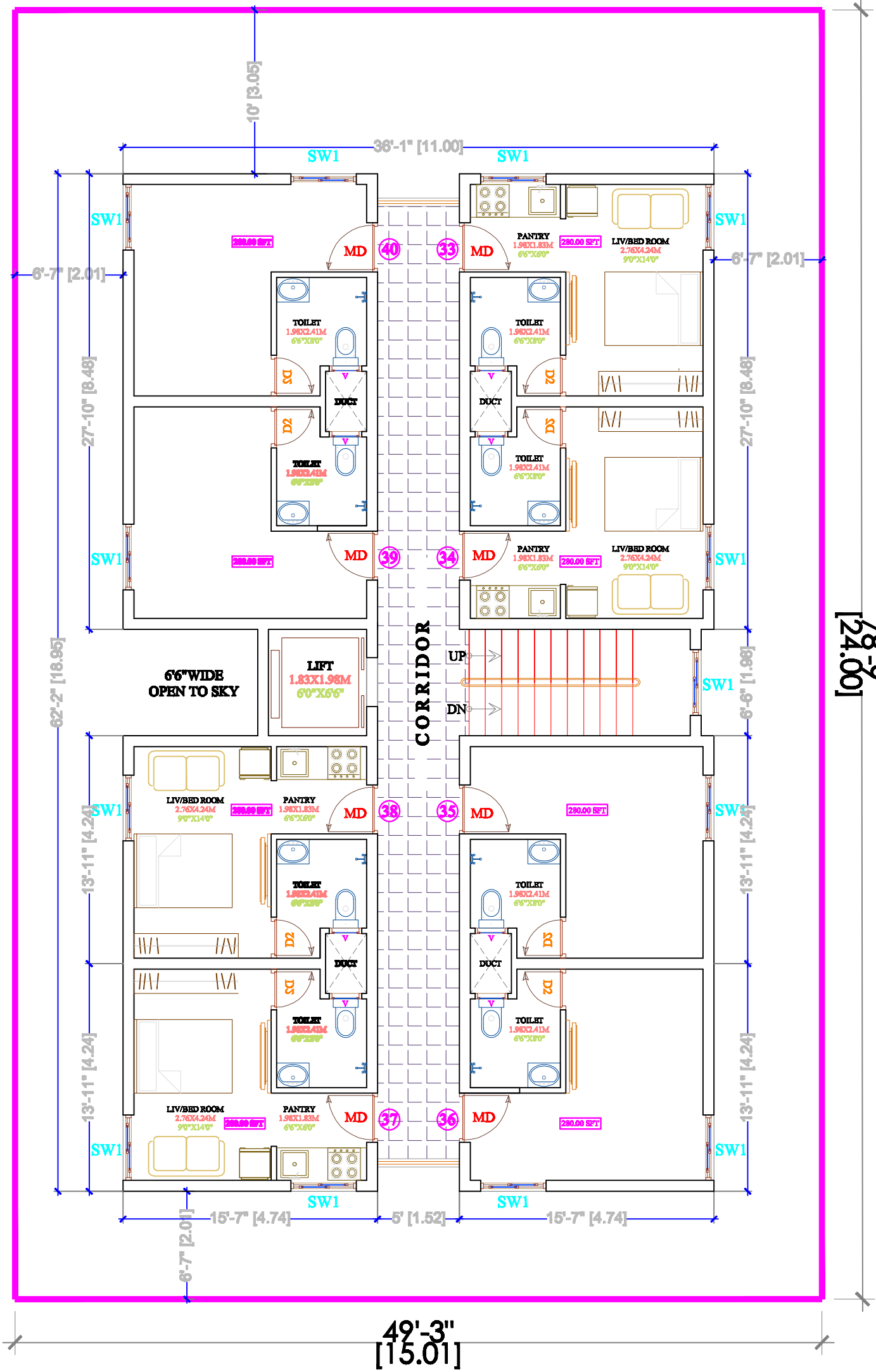
5TH FLOOR PLAN
